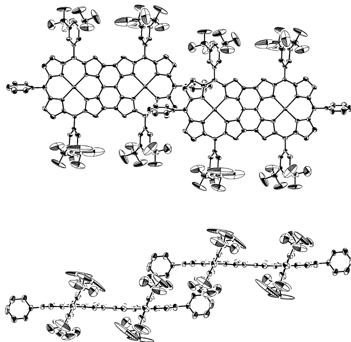
Figure 2. Molecular structure of 9 . Top: top view; bottom: side view. Hydrogen atoms, benzene, and ethanol molecules are omitted for clarity.
